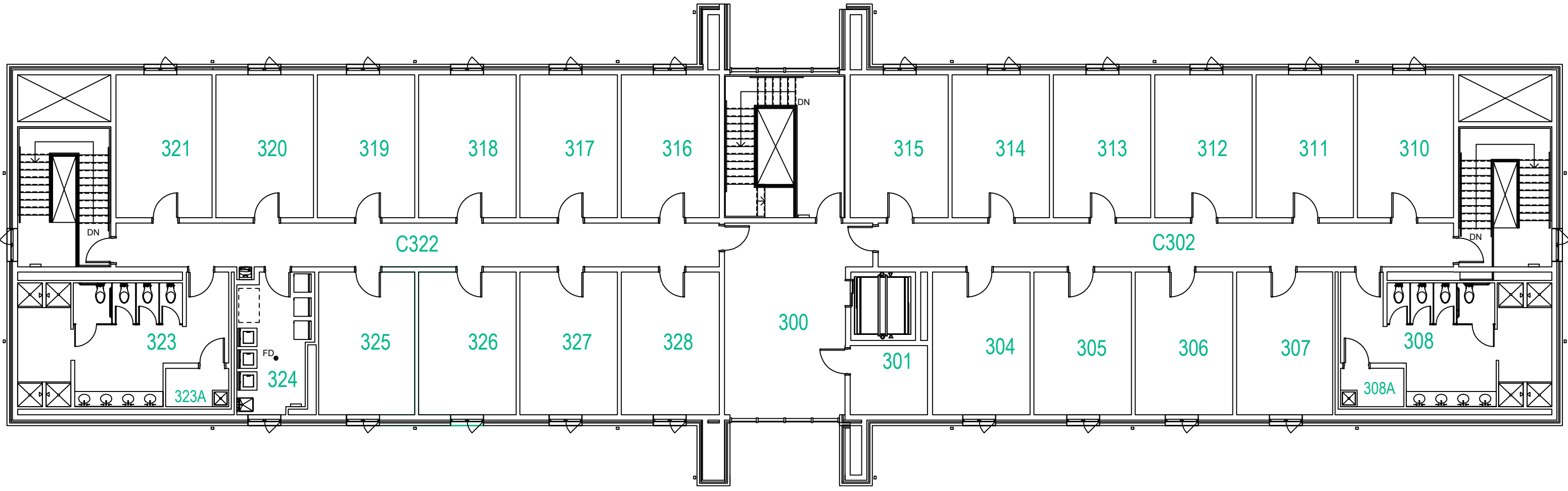
ARCHITECTURAL THIRD FLOOR PLAN
