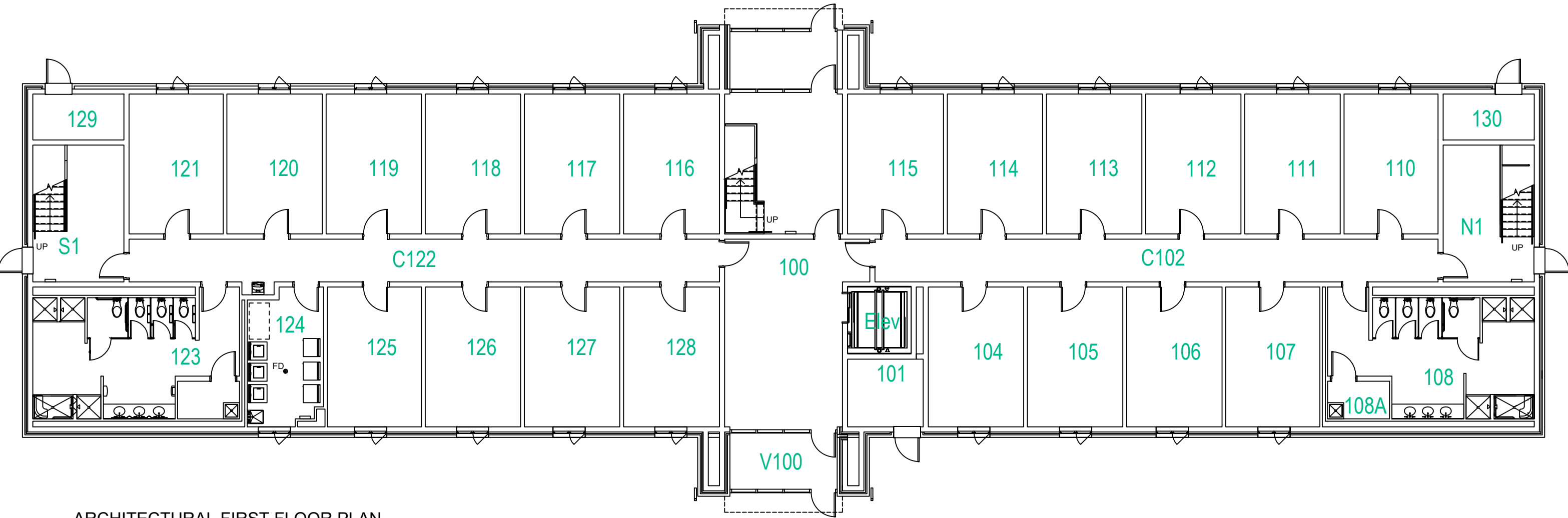
ARCHITECTURAL FIRST FLOOR PLAN
